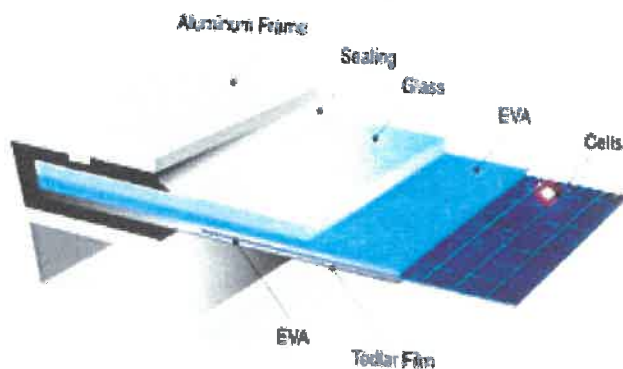
Figure 2: Components of crystalline silicon panels. The vast majority of silicon panels consist of a glass sheet on the topside with an aluminum frame providing structural support. Image Source: www.riteksolar.com.tw
